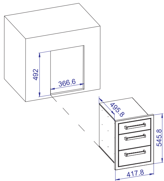
Cutout Size
