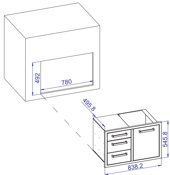
Cutout Size
