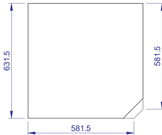
Vertical View
